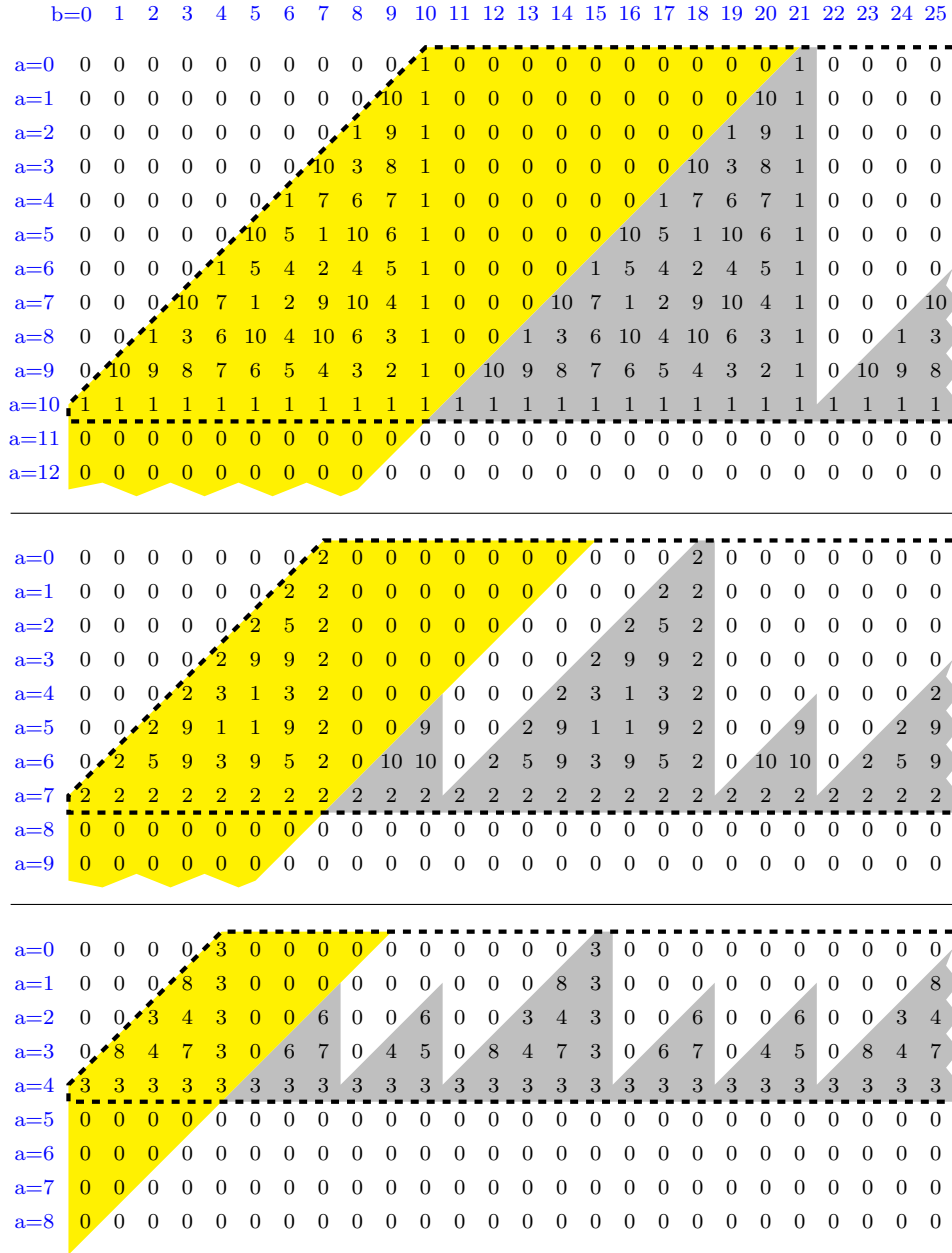
FIGURE 1. Tables of S_1(a, b, -) , S_2(a, b, 3) , S_3(a, b, 3) values for p = 11 and small integers a, b . Yellow shading indicates the range covered by Theorem 4.1, and the dotted lines enclose the region covered by Theorem 5.1. The structure of the gray shading is discussed in Section 5.3.
